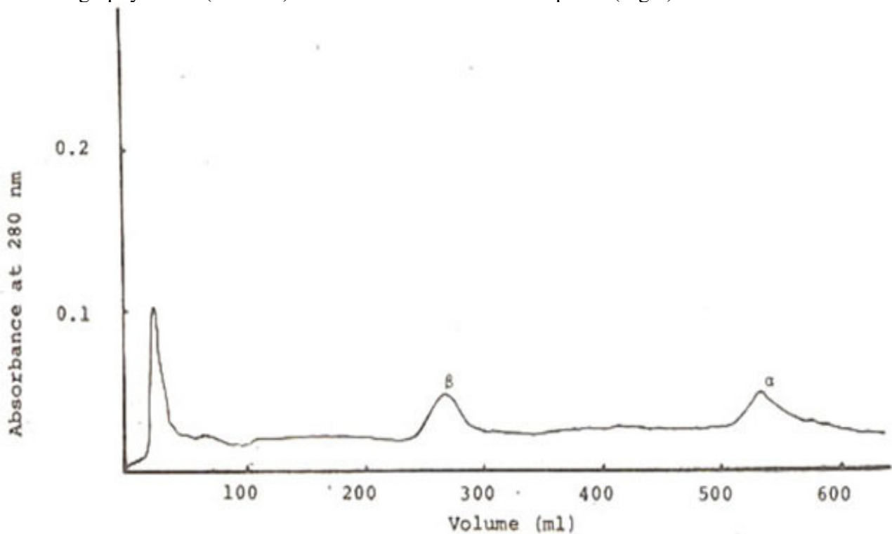
Figure 2. Separation of the polypeptide chains from Hb (Karachi) on CM-Cellulose column. Elution buffer: 8M Urea + 0.05M 2-Mercaptoethanol + 0.01M \text{Na}_2\text{HPO}_4 ; pH 6.5-7.2.
