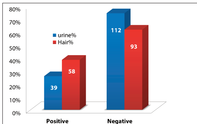
Figure-1: Qualitative results for cannabis in urine and hair samples of 151 subjects.
